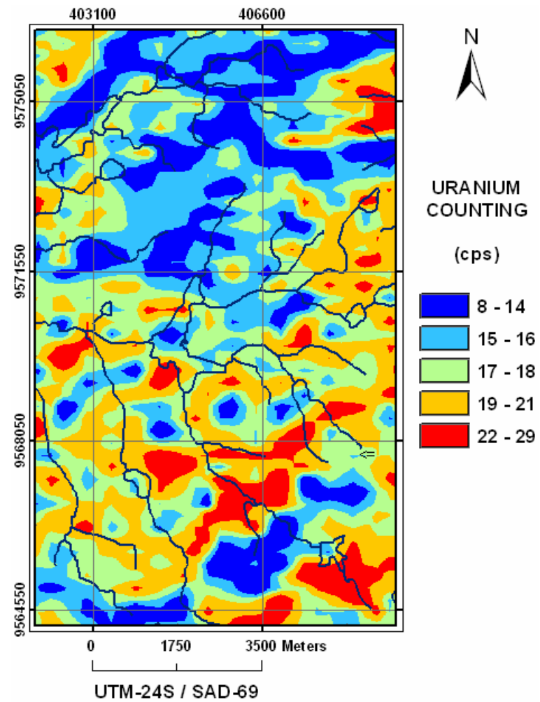
Figure 3.7 – Itatira-B radiometric data resampled on 25-m cell-size grid and trimmed to Juá study-area. Uranium intensity in counts per second. Drainage and reservoirs are indicated by blue lines.
