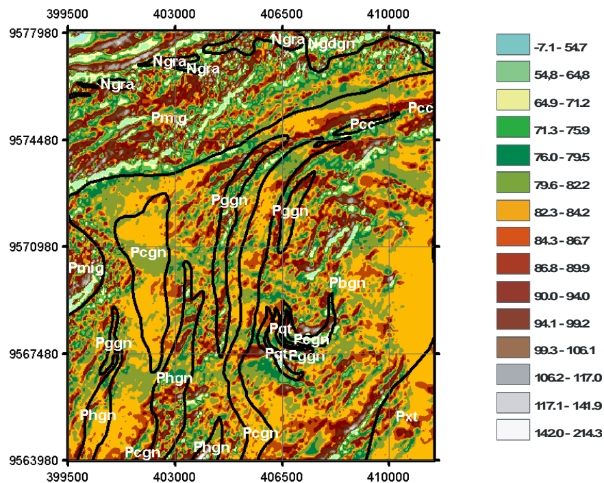
Figure 3.30 - Reclassified filtered 60 m-depth magnetic data (nT) overlaid by the geologic map of Juá. Note the correspondence of migmatite (Pmng) with alternate high- and low- magnetic anomaly classes, and the calc-silicate gneiss with moderate magnetic classes.
