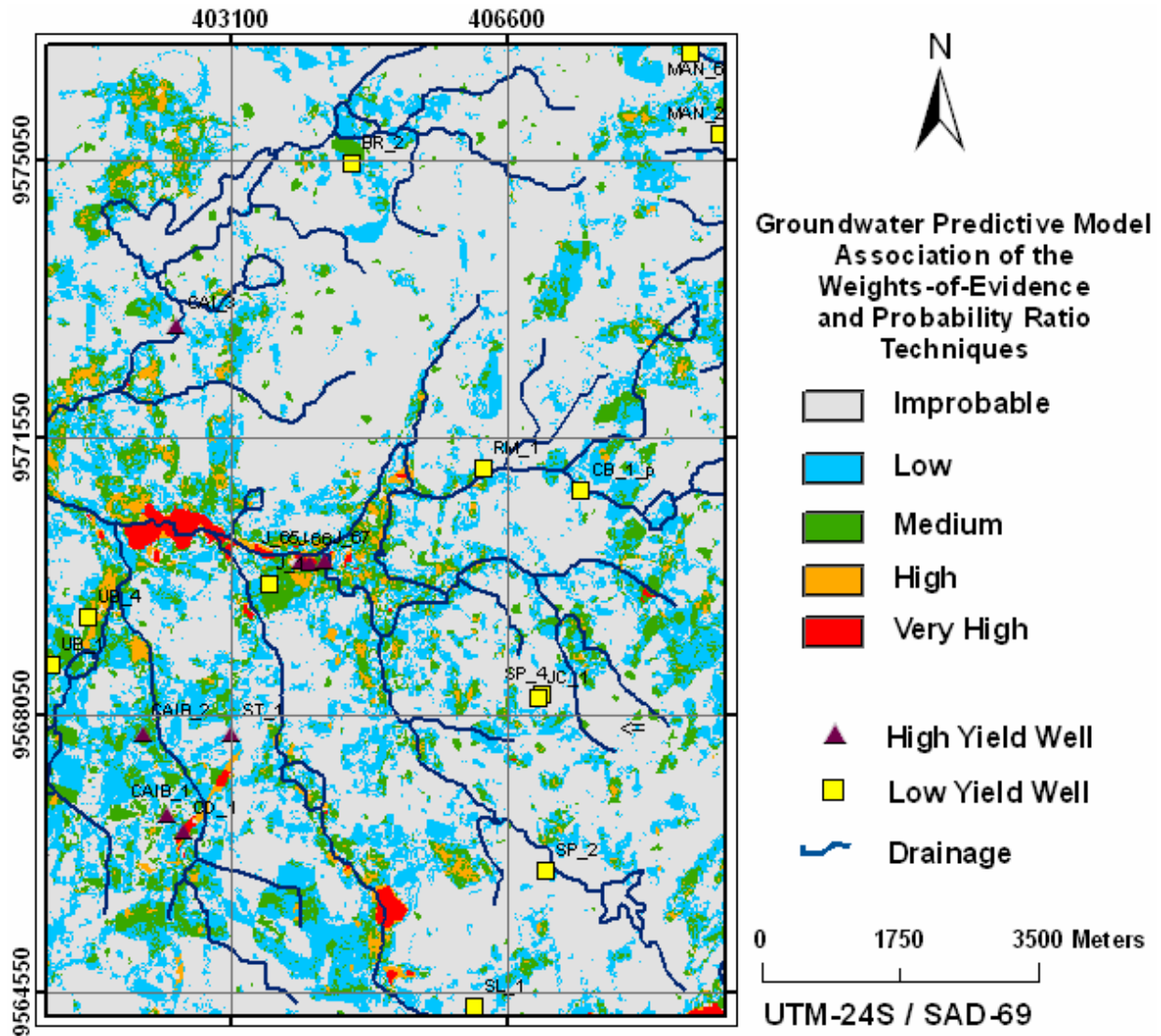
Figure 5.14 - Combined map between the five favorability classes of WofE model A2 and the yield class 4-Pr model, according to the conditional operator of Either Pr-WofE IF Pr>WofE ELSE WofE. Regions not mapped as favorable in WofE model (e.g. northwestern area) were better ranked.
