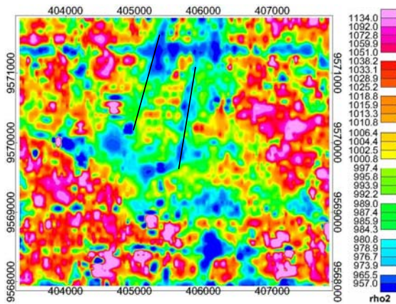
b) Bottom-layer resistivity (ohm-m)
