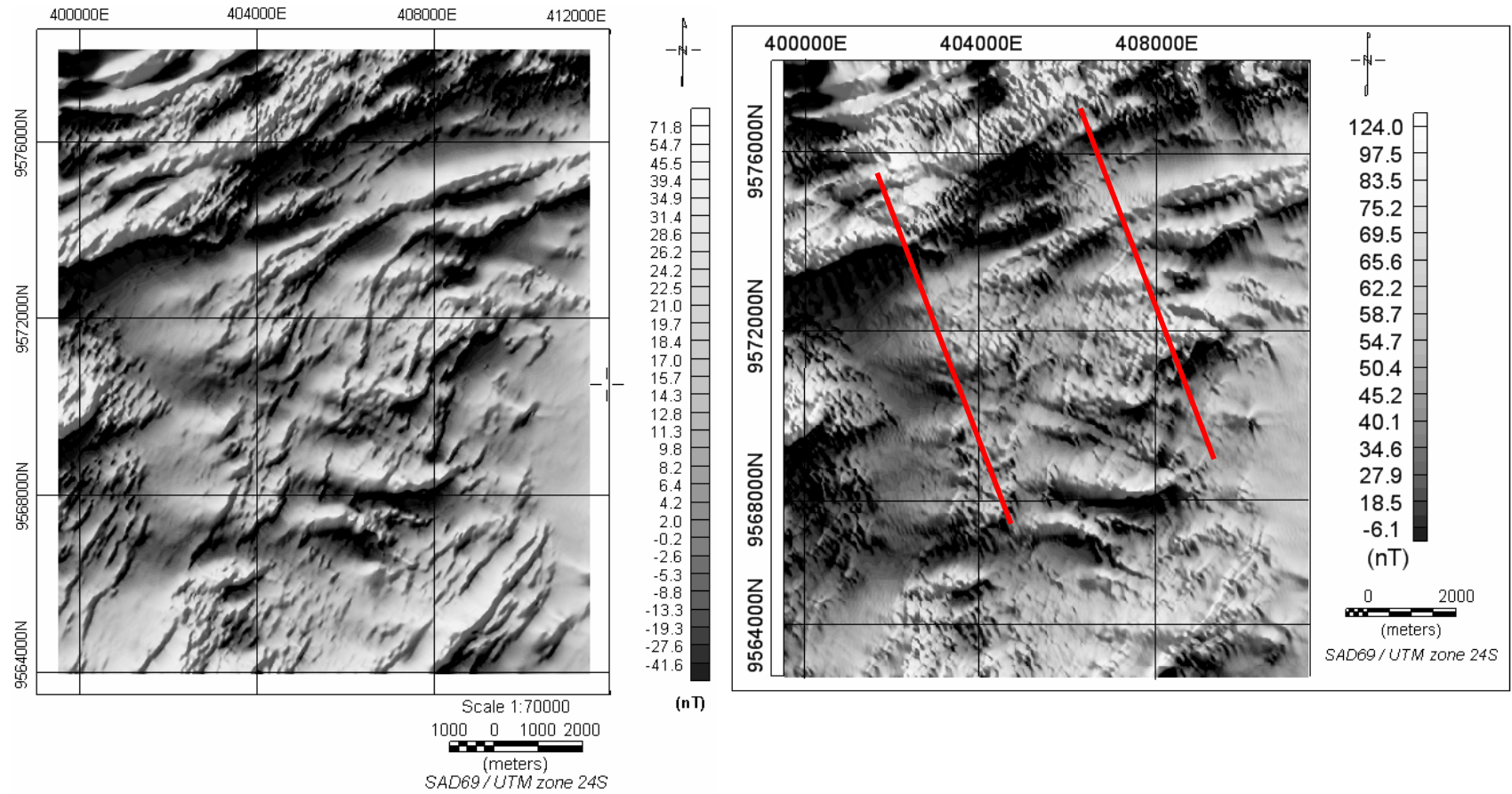
Figure 3.8 – Comparison of reductions to magnetic north pole filters applied on Juá magnetic residual field grid: a) good result using Phillips (1997) algorithm with amplitude correction of 79.11^\circ ; b) bad result using Oasis Montaj algorithm with amplitude correction of 70^\circ plus a cosine low-pass filter at 130^\circ Azimuth. Red traces mark artifacts with direction parallel to the geomagnetic declination, generated after the application of Oasis Montaj's algorithm.
