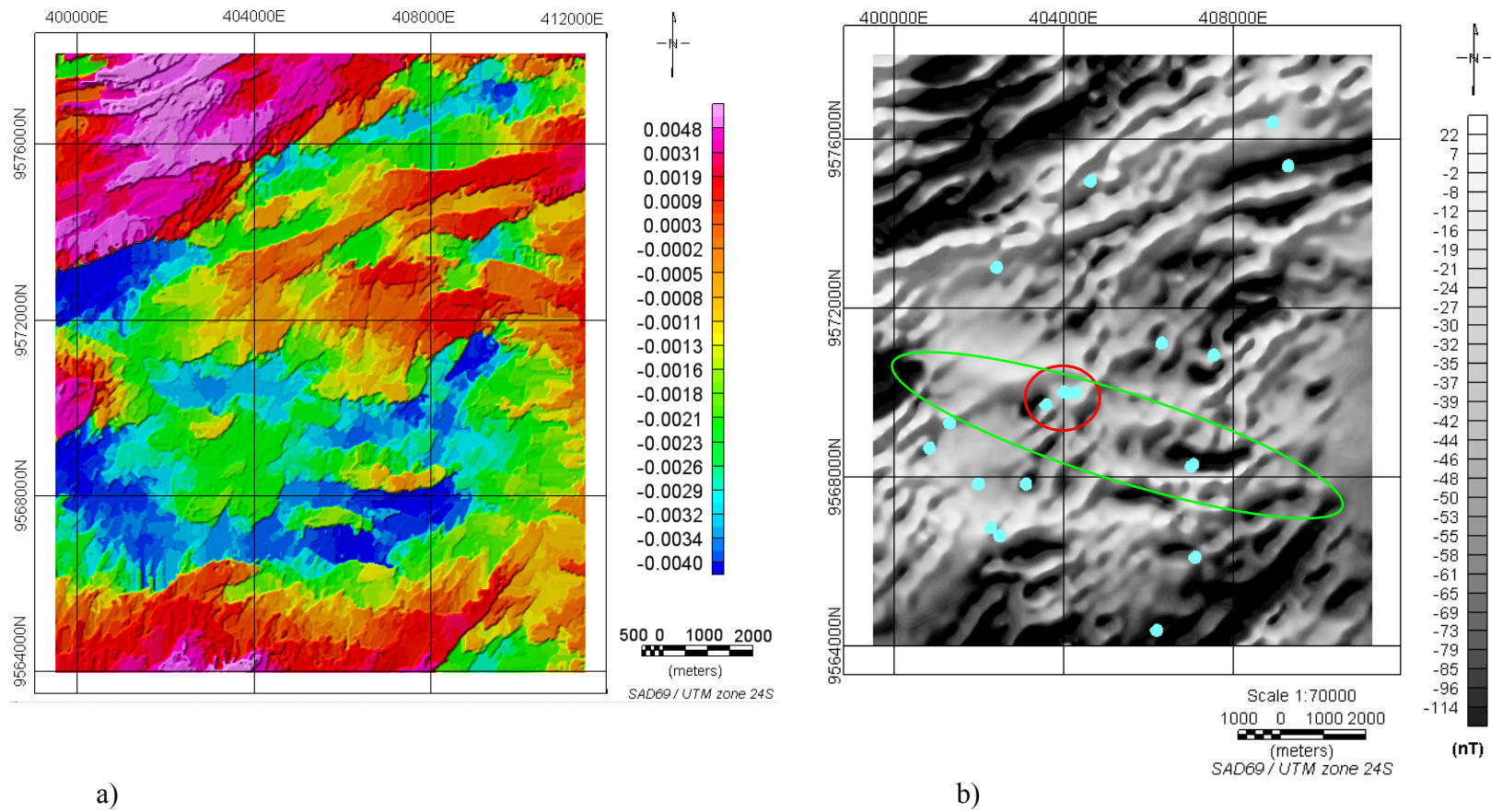
Figure 3.12 - Juá high-resolution magnetic data processed as: a) Terrace-magnetization map using the terracing technique of Cordell and McCafferty (1989), and b) High-resolution 2000-m-depth layer grid after the subtraction of the regional 2000-m-depth grid from higher-resolution anomaly grid. The dots represent locations of drilled water-wells. Note that in the map (b), the most productive wells (surrounded by a red circle) are in the border of an important negative gradient, oriented WNW-ESE (marked by a green ellipse).
