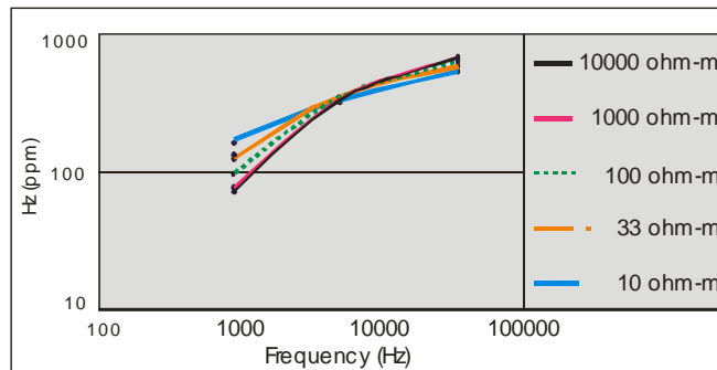
b) Quadrature sensitivity to basement resistivity.
