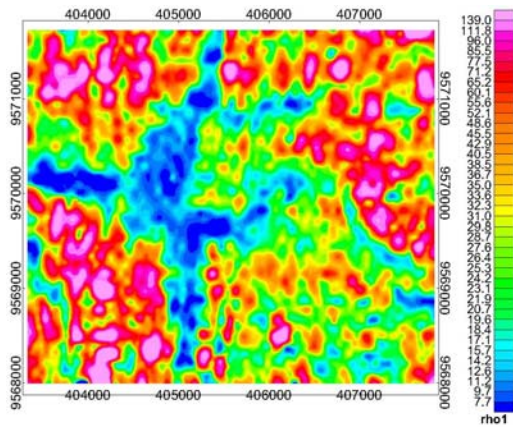
a) Top-layer resistivity (ohm-m)
