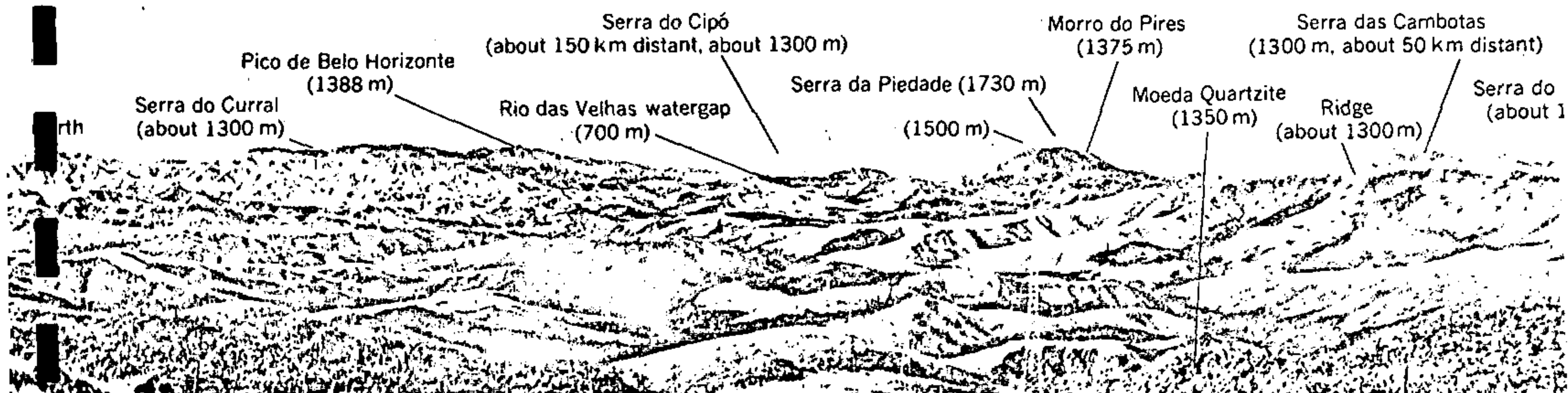
FIGURE 4.—Panoramic view from near N. 3,200 E. 6,550, Macacos quadrangle, looking from north to nearly east. Camera elevation is 1,400 m. Crags in the foreground are Moeda quartzite; dissected rocks of the Nova Lima Group are in the middle distance; ridgelines on the horizon are Minas Series rocks. Serra da Piedade is 40 km, and Pico de Belo Horizonte about 20 km, from camera. Rio das Velhas, the master stream, flows in entrenched meanders behind Morro do Pires northward through the watergap in the Serra do Curral.
