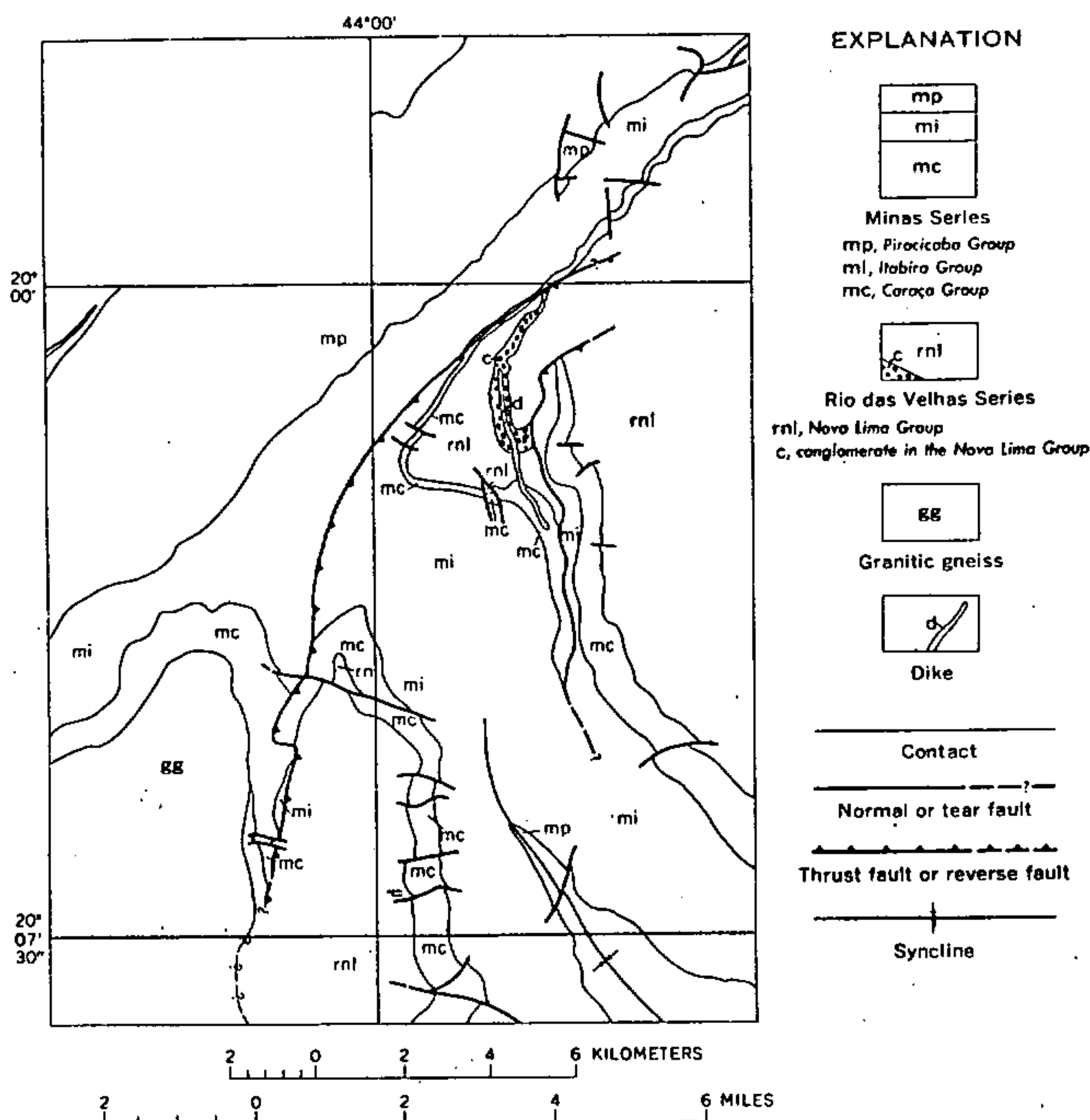
FIGURE 26.—Alternative explanation of structure at junction of the Moeda syncline with the Serra do Curral, to be compared with plate 1. See plate 1 for structural details, topography, and drainage.
