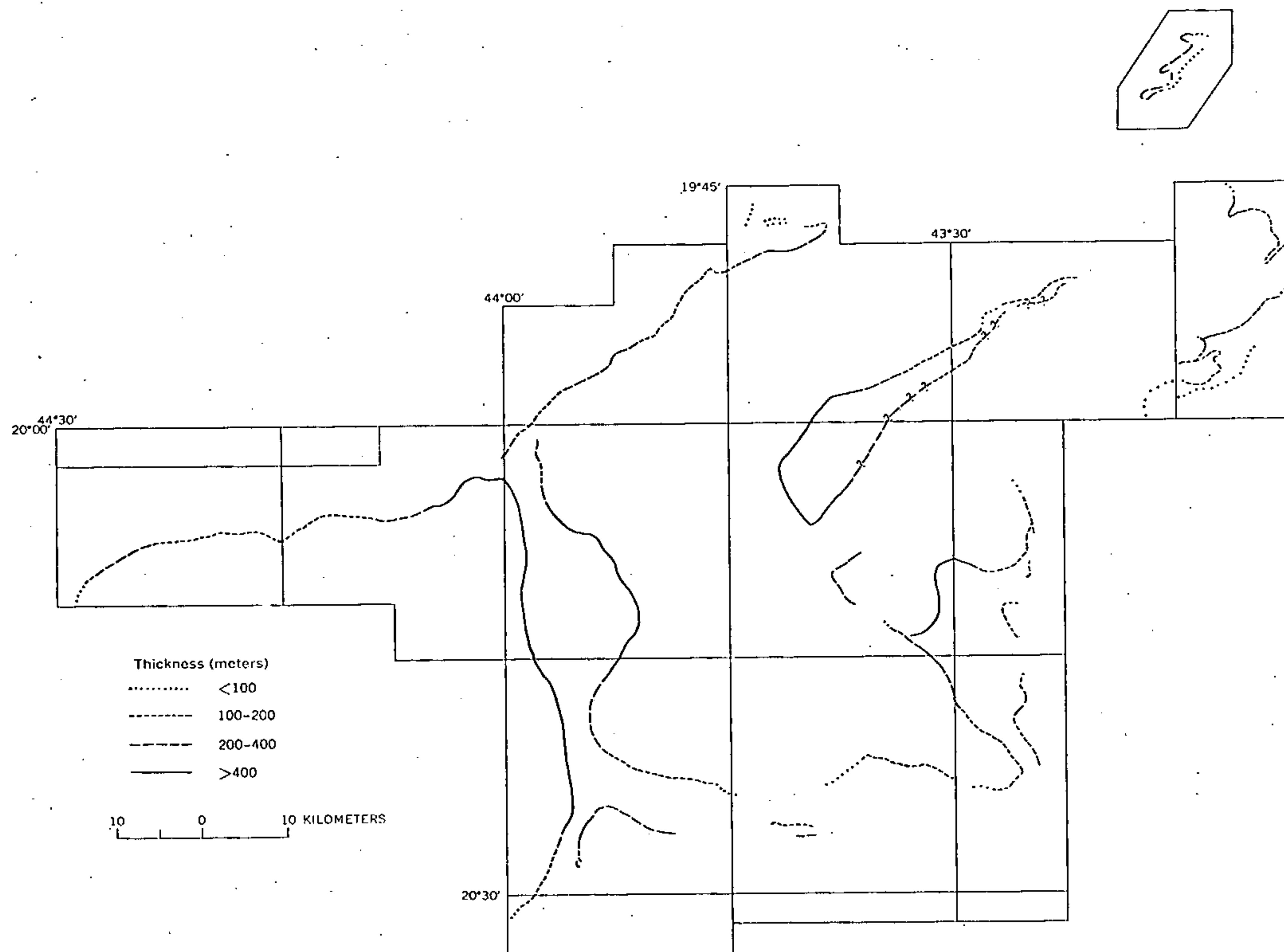
FIGURE 12.—Regional variations in thickness of the Cauê Itabirite.
