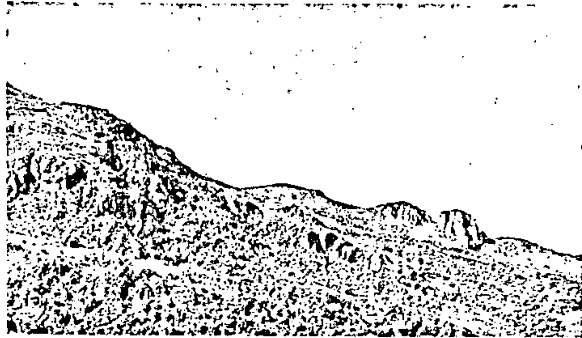
FIGURE 7.—Typical cliffy outcrops of the Cambotas Quartzite in the Serra das Cambotas, Santa Bárbara quadrangle.
