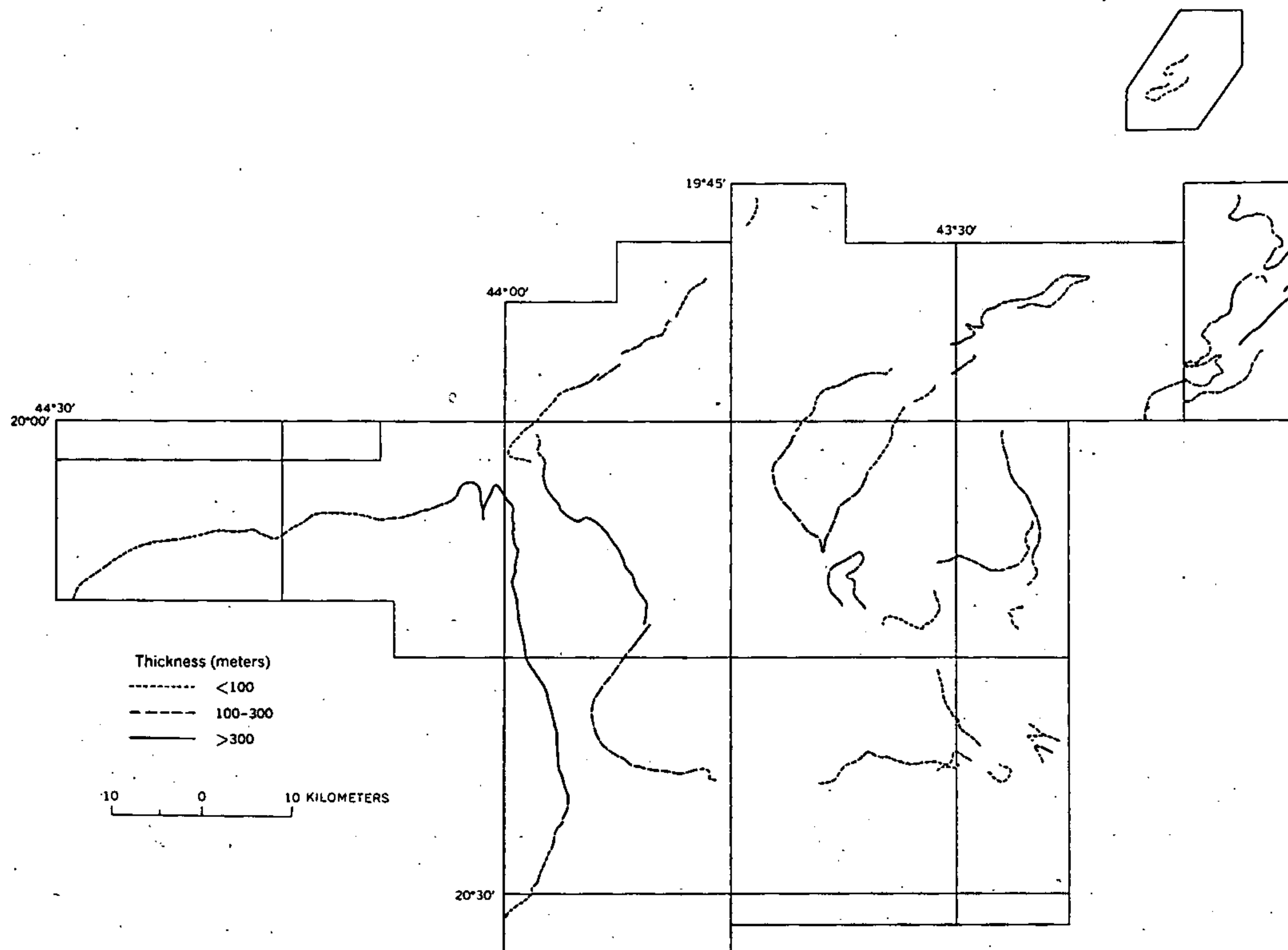
FIGURE 8.—Variations in thickness of the Moeda Formation in the Quadrilátero Ferrífero. Thickness shown is only approximate; local tectonic deformation obscures the true stratigraphic thickness in many places.
