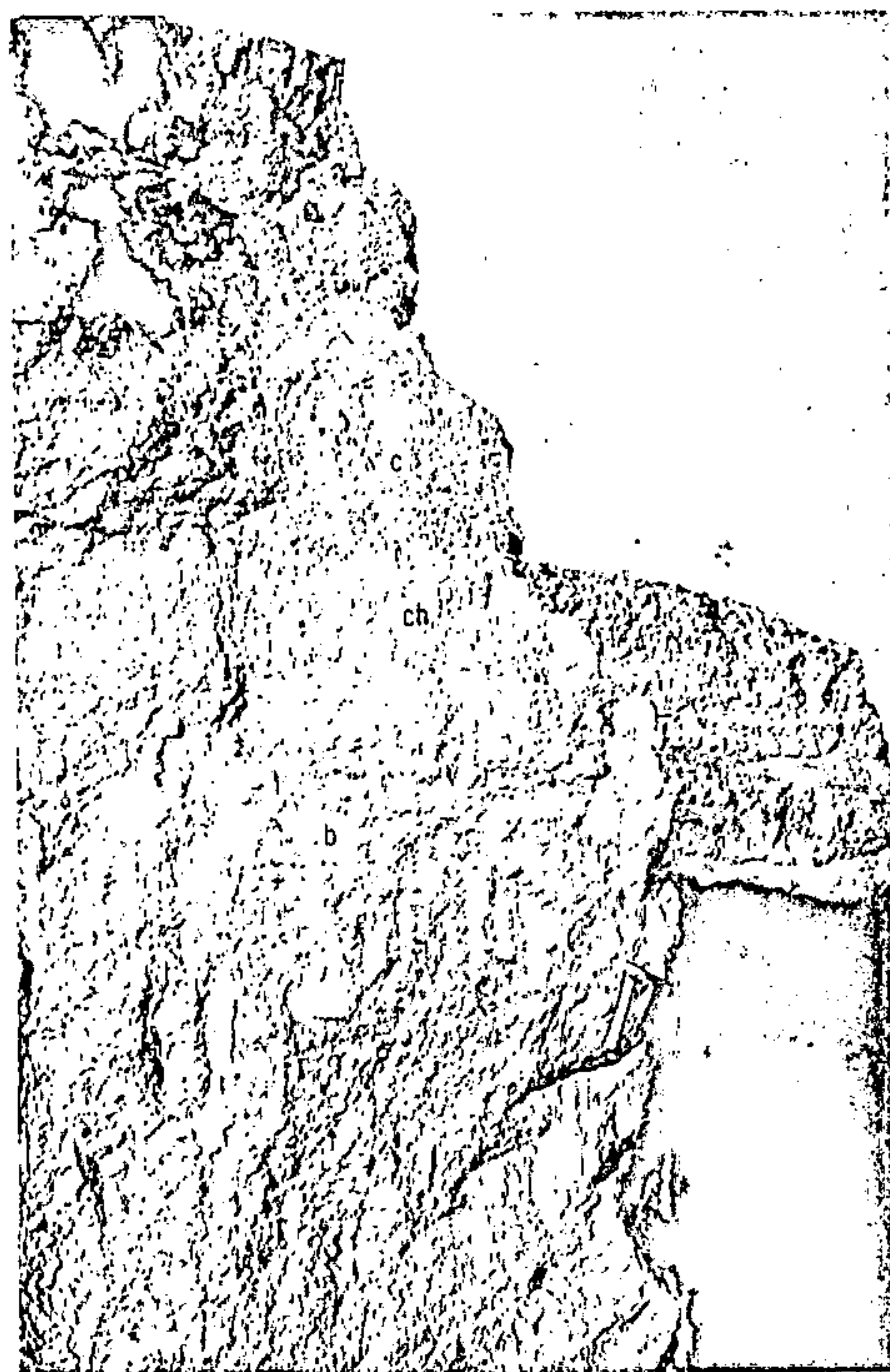
FIGURE 21.—Laterization profile, Mutuca bauxite mine, N. 8,000, E. 2,500, Muencos quadrangle. The uppermost zone is chemical canga (c). The next zone is light-brown to tan highly aluminous and ferruginous hard canga (ch), with strongly marked vertical flutings. Beneath the canga is a zone of pink to buff commercial bauxite (b) 1–3 m thick. The hammer is in bauxite. Below the bauxite is a varying but usually thick high-alumina clay, at least 10 m thick in this area. Here the chemical canga at the top may well be somewhat younger than the underlying zones and unrelated to them in genesis.
